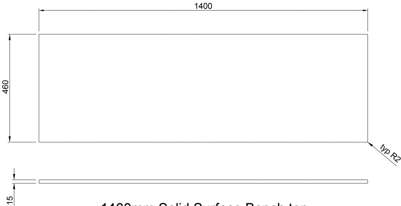
1400mm Solid Surface Bench top
