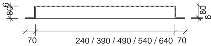
Section
