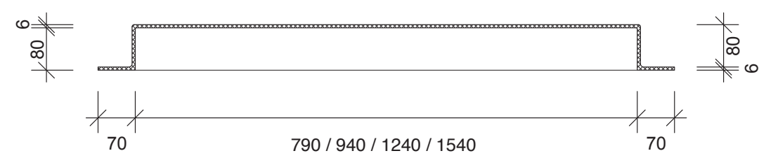
Section
