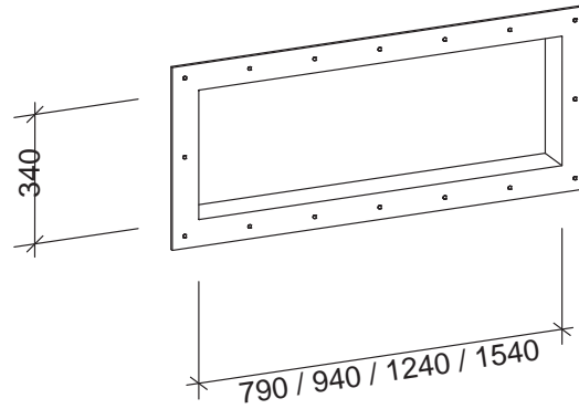
Perspective
