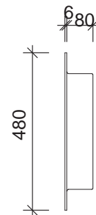
Side Elevation
