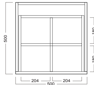
Side Section
