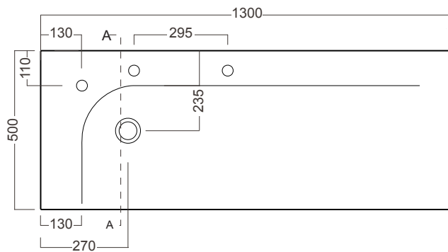
WASHBASIN TOP VIEW
