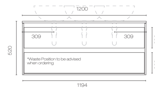
1200mm (2 Drawer)
