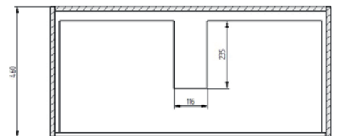
Section of Top Drawer
