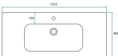
Top & Basin Top Down
