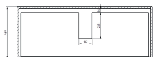
Section of Top Drawer
