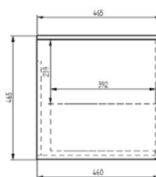
Side Section
