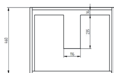
Section of Top Drawer
