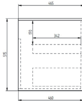
Side Section
