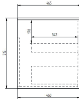
Side Section
