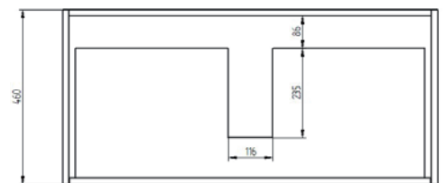
Section of Top Drawer
