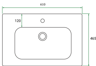
Top & Basin Top Down
