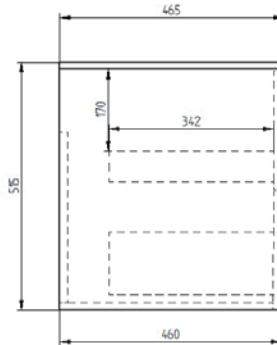
Side Section
