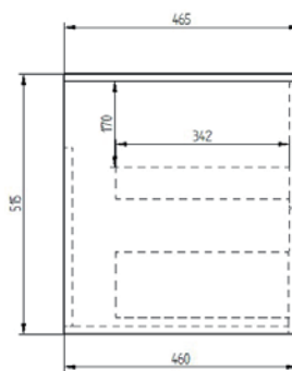
Side Section
