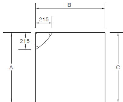
Top View (Generic - 3 sided)
